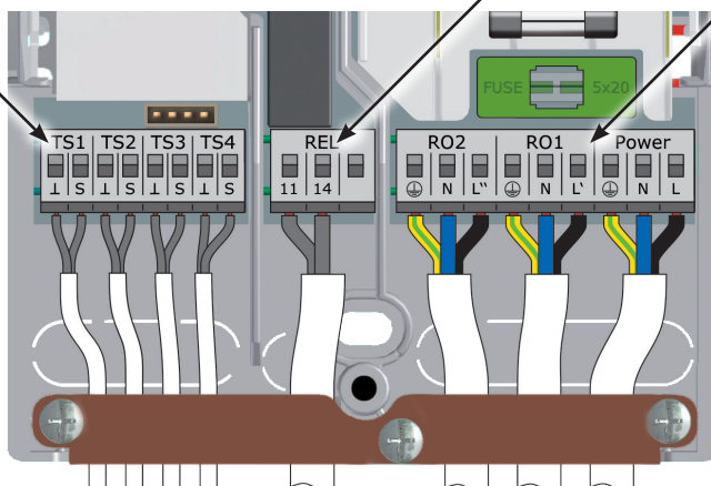
Morsettieria REL
