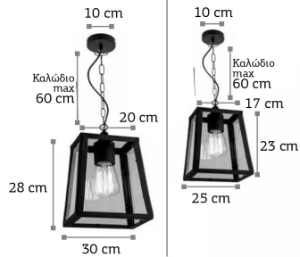
4420A 1xE27 11-58-00 4420B 1xE27 11-48-00
