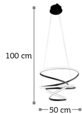
6148A LED 68watt 3000K 5100Lm 11-201-50
